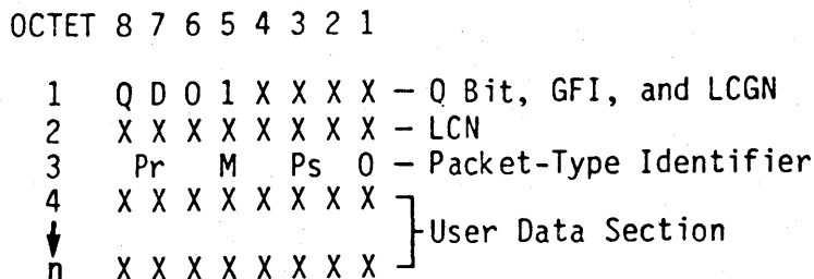
Figure 9-6. DTE and DCE Data Packet Format
