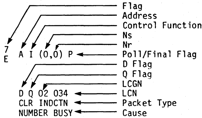
Figure 9-14. Typical Display Format
