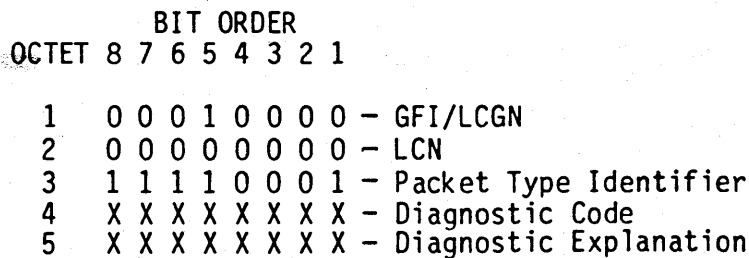
Figure 9-12. DCE Diagnostic Packet Format
